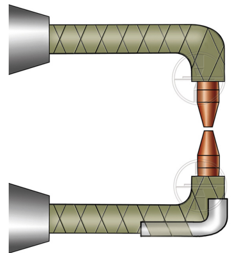
Isolier-Schutzbinden
